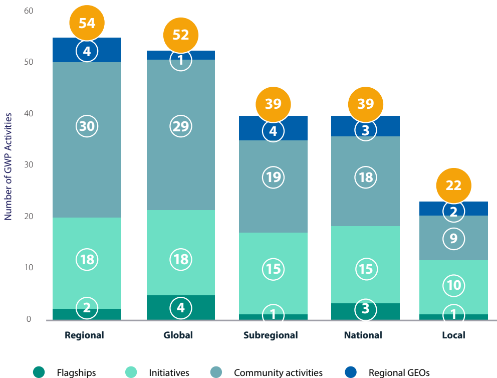
Fig.6 - GWP activities impact across geographies per type of activity
