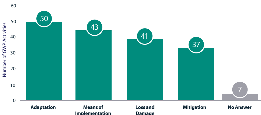
Fig.14 - Climate action workstreams supported by GWP activities
